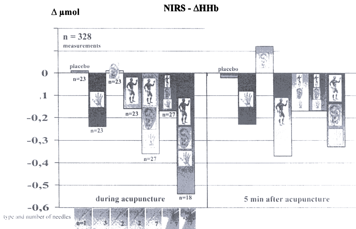
Fig. 5. Cerebral changes (generally decreases) in desoxyhemoglobin (HHb). For further descriptions see Fig. 4.
