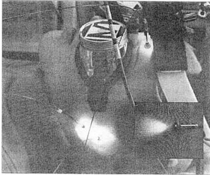
Fig. 1. Test person during laserneedle stimulation and simultaneous registration of NIRS parameters. Right bottom: single active laserneedle and application device.
