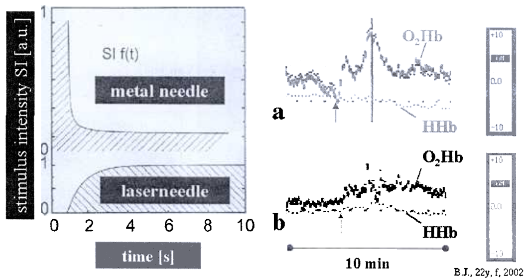
Fig. 3. Left: Stimulus intensity ( SI f(t) ) as a function of time (hypothesis). Right: Real measured cerebral responses of NIRS-parameters O_2Hb (oxyhemoglobin) and HHb (desoxyhemoglobin) on manual, brief (20 seconds) acupuncture needle stimulation (a) and laserneedle stimulation (b) in 22-year-old female test person. The arrows indicate the beginning of stimulation.
