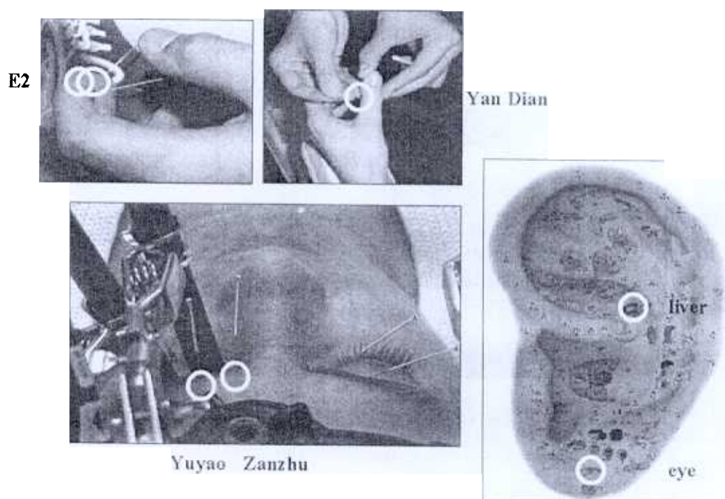
Fig. 2. Acupuncture schemes used in this study.
